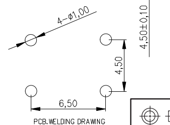
PCB.WELDING DRAWING
