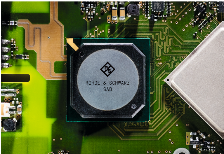
The Rohde&Schwarz designed 10-bit A/D converter ensures highest signal fidelity at highest resolution
