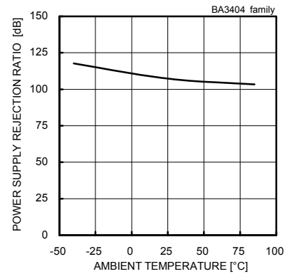
Fig. 15 Power supply rejection ratio – Ambient temperature (VCC/VEE=+15[V]/-15[V])
