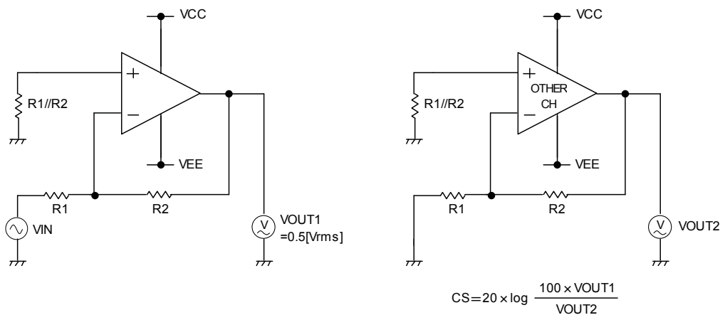
Fig5. Test circuit3
