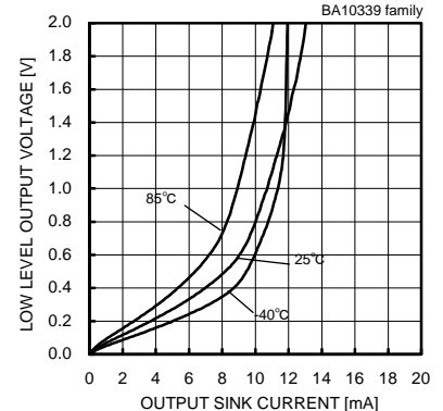
Fig. 26 Low Level Output Voltage - Output Sink Current (VCC=5[V])
