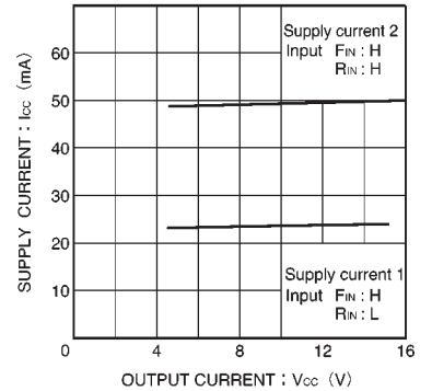
Fig.8 Supply current vs.output current
