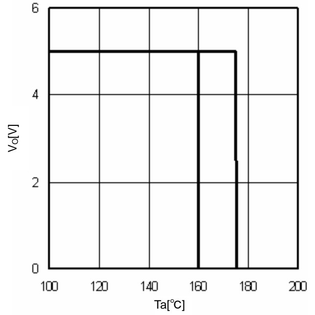
Fig.15 TSD ( I_o=0mA )
