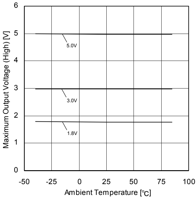
Figure 31. Maximum Output Voltage (High) vs Ambient Temperature (R L =20kΩ)
