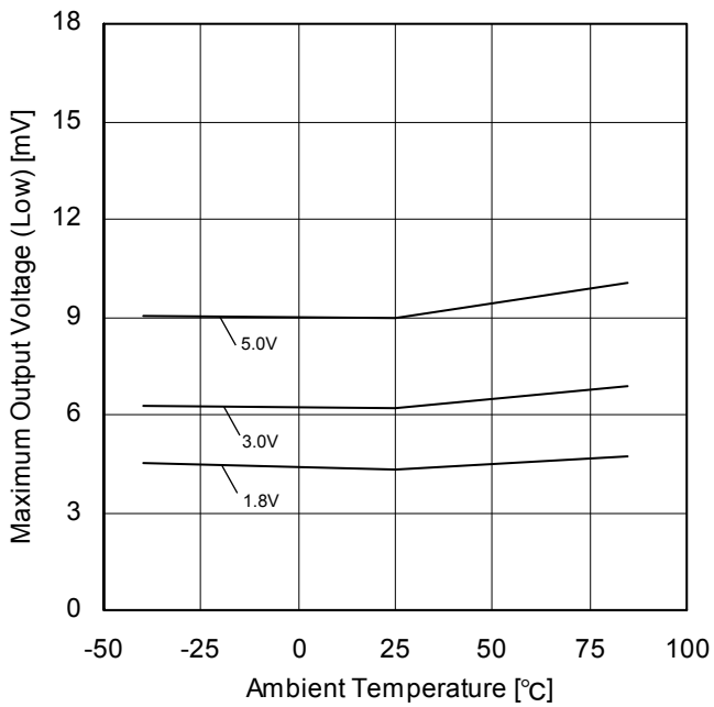
Figure 33. Maximum Output Voltage (Low) vs Ambient Temperature (R L =20kΩ)
