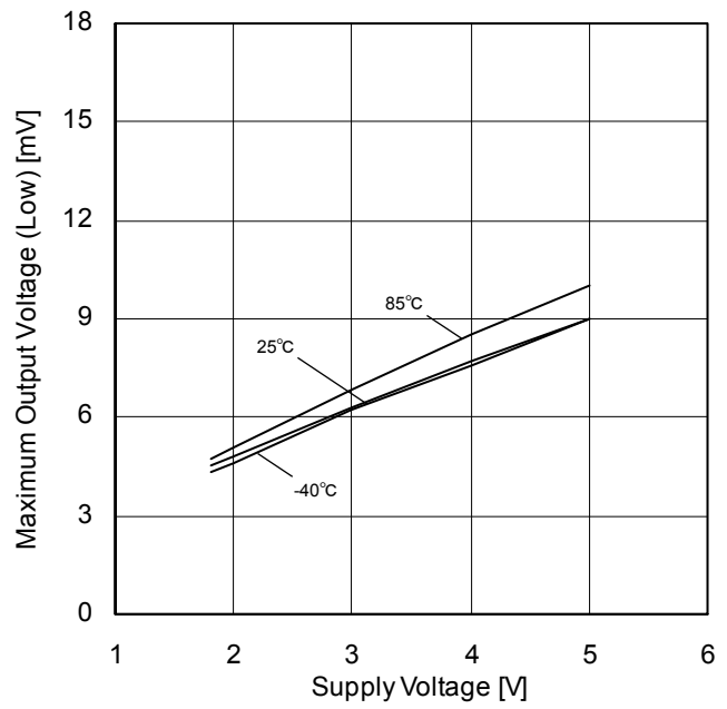
Figure 32. Maximum Output Voltage (Low) vs Supply Voltage (R L =20kΩ)
