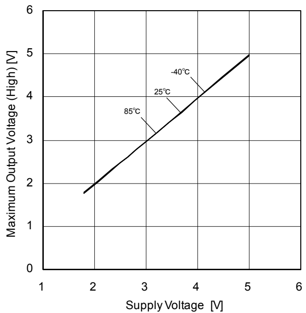
Figure 34. Maximum Output Voltage (High) vs Supply Voltage (R L =2kΩ)
