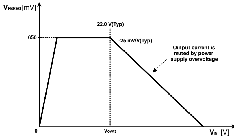
Figure 29. Over Voltage Mute Function (OVM)
