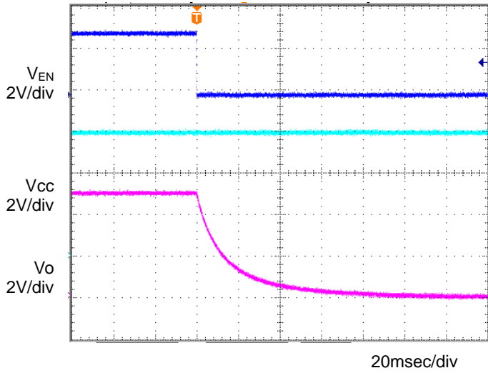
Figure 19. OFF sequence 2 Co=1μF, Ta=25°C
