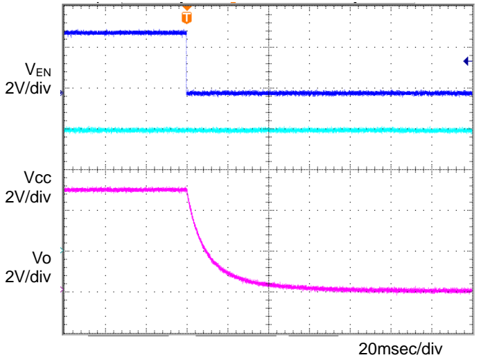
Figure 20. OFF sequence 2 Co=1μF, Ta=105°C
