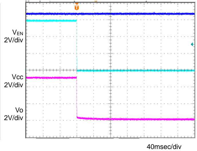
Figure 14. OFF sequence 1 C_o=1\mu F, T_a=105^\circ C
