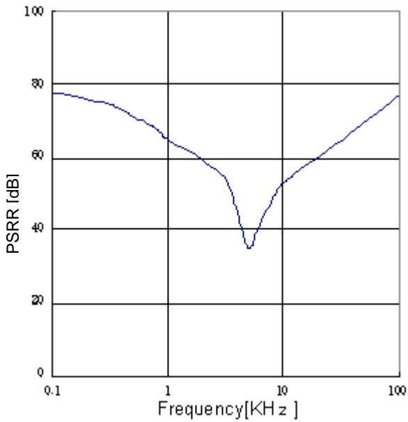
Figure 33. PSRR (Io=0mA)
