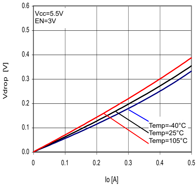
Fig.37 Minimum dropout Voltage 4 (V CC =5.5V)
