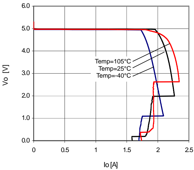
Figure 29. OCP
