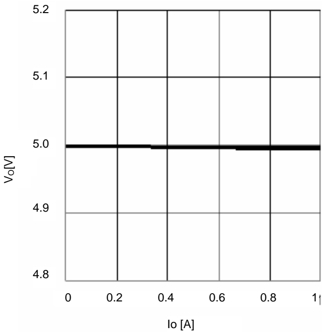
Figure 25. I_O - V_O
