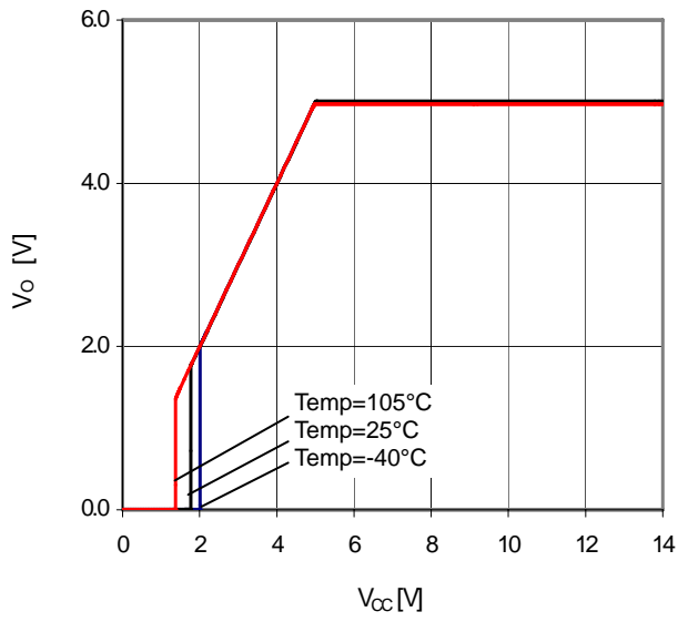
Figure 27. V_{CC}-V_o ( I_o=0mA )
