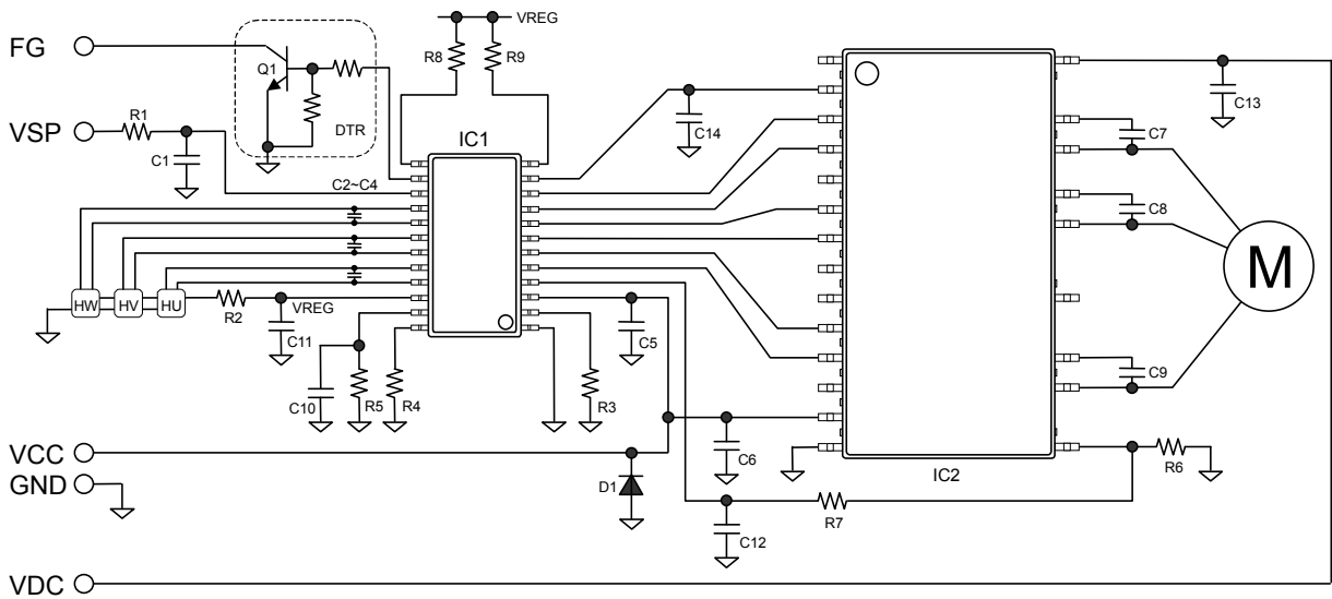
Figure 33. Application circuit example (150° commutation driver)
