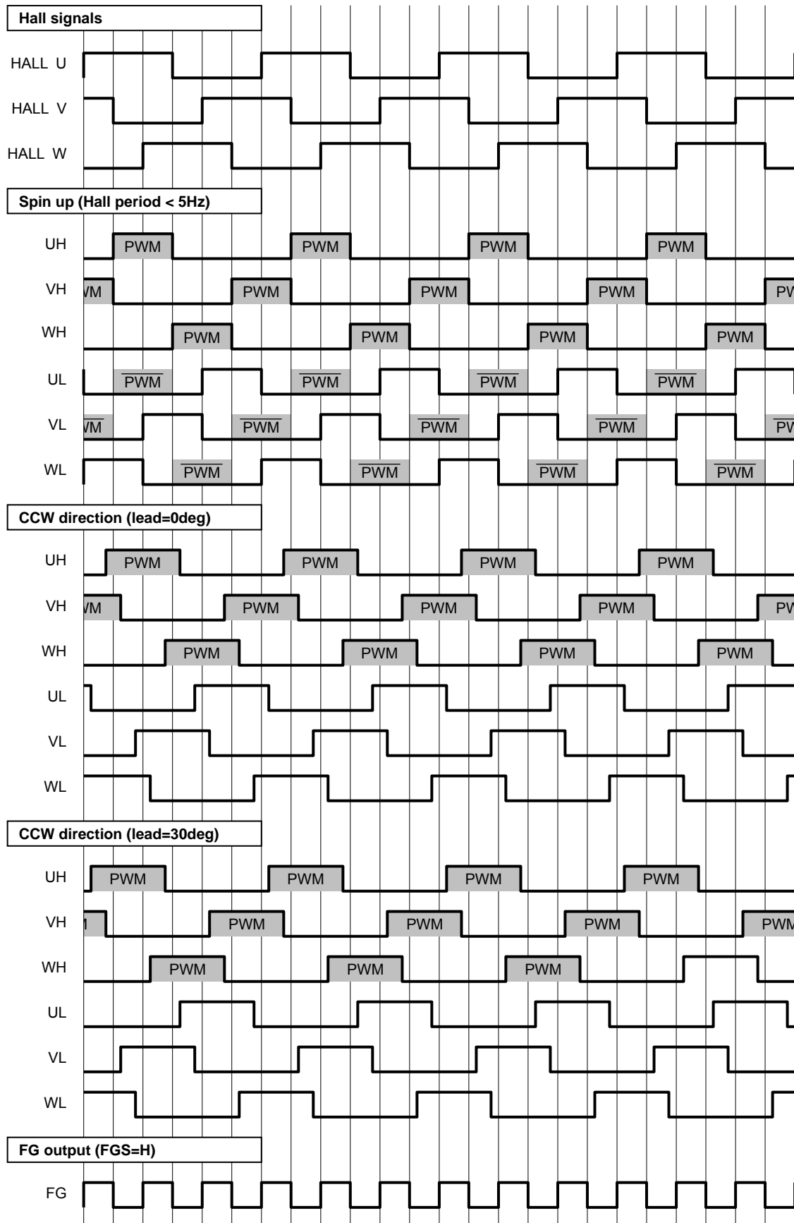
Figure 8. BD62012AFS (Counter clockwise) timing charts
