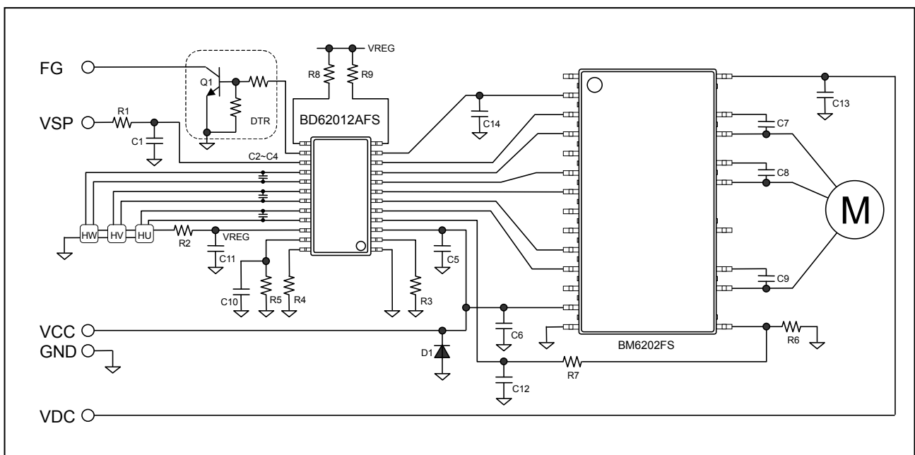
Figure 1. Application circuit example - BD62012AFS & BM6202FS
