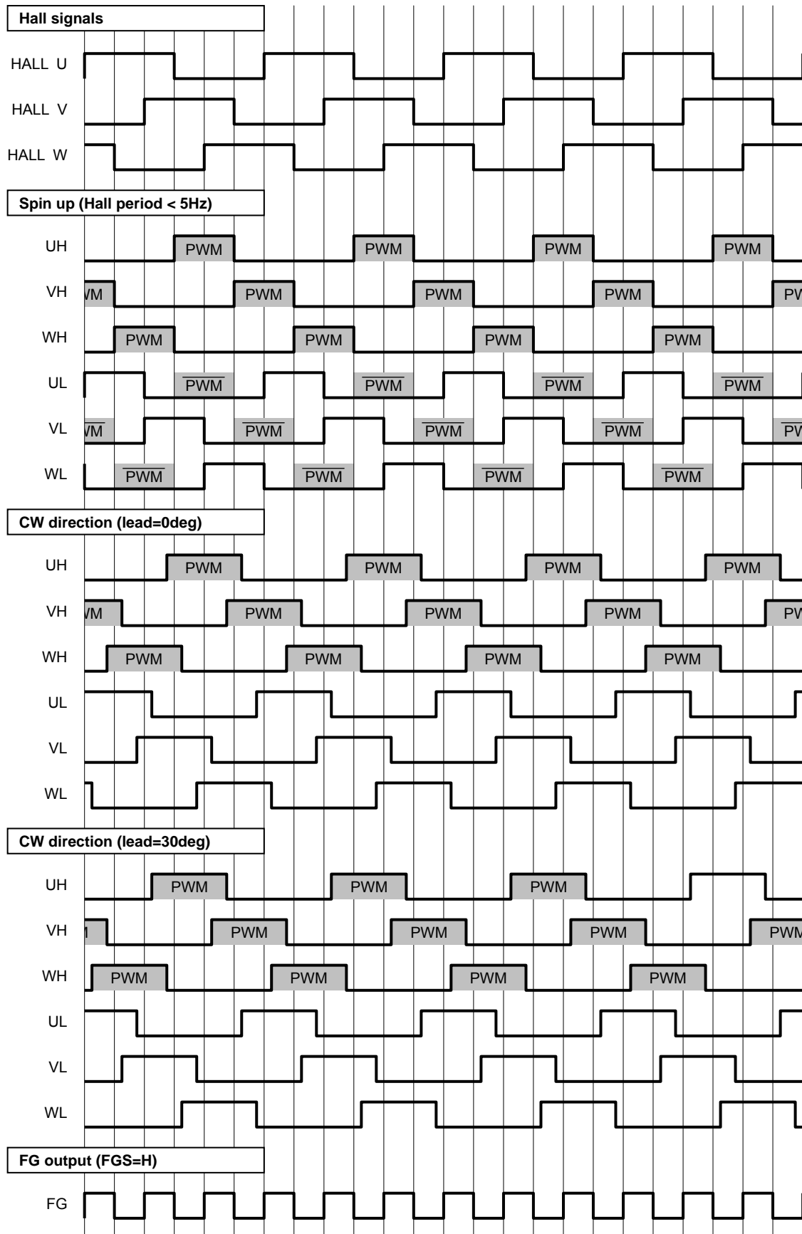
Figure 7. BD62012AFS (Clockwise) timing charts
