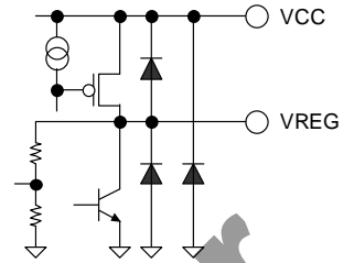
Figure 37. VREG, VCC
