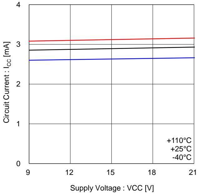
Figure 7. Quiescence Current
