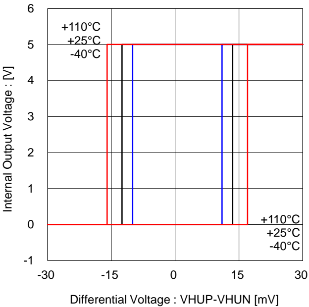
Figure 13. Hall Comparator Hysteresis Voltage
