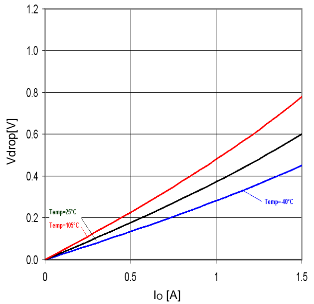
Fig.34 Minimum dropout Voltage 2 (Vcc=4.5V、Ta=25°C)
