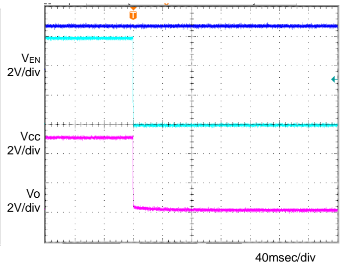
Fig.14 OFF sequence 1 C_o=1\mu F, T_a=105^\circ C
