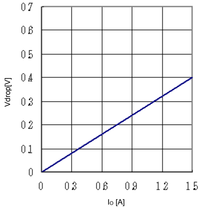
Fig.24 Minimum dropout Voltage 4 (V CC =8V, T a =25°C)
