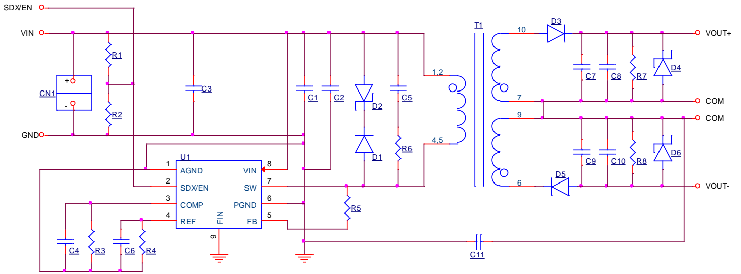
Figure 4. BD7F100HFN-EVK-003 Circuit Diagram
