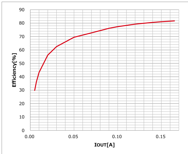
Figure 13. Efficiency vs Load Current
