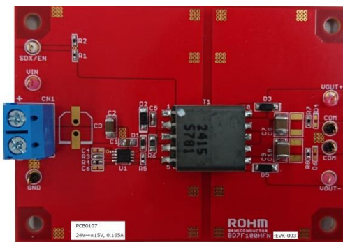
Figure 1. BD7F100HFN-EVK-003 Evaluation Board
