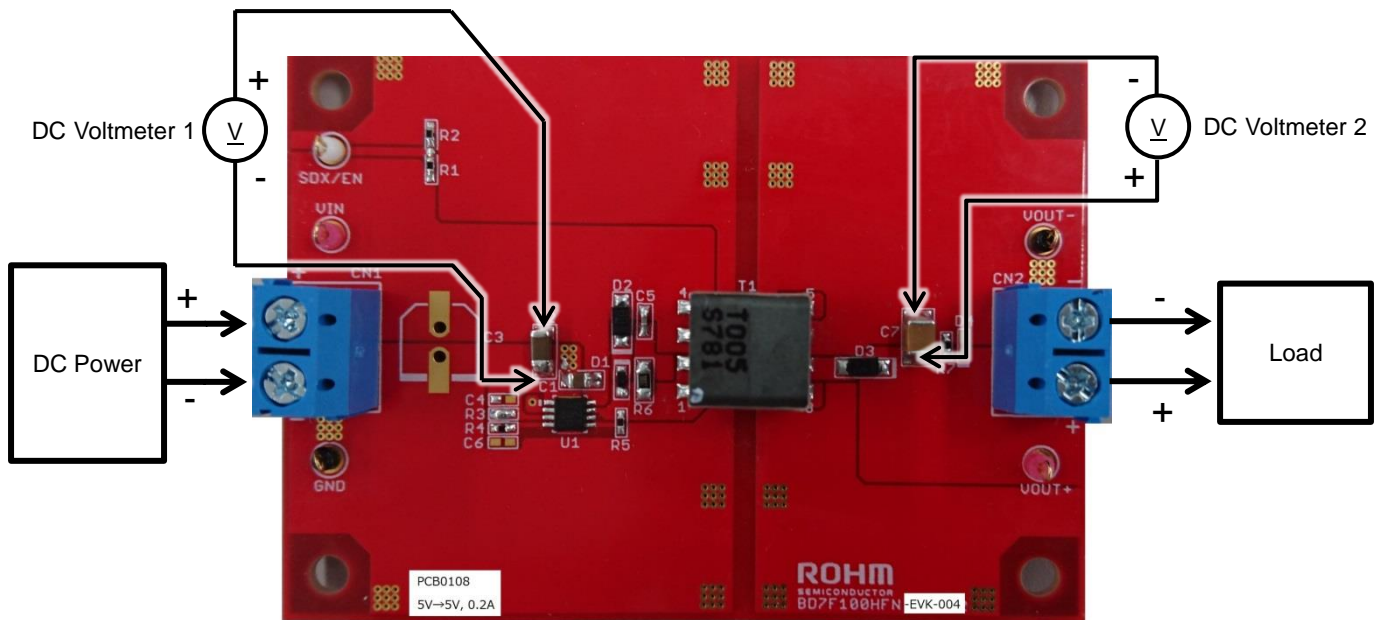
Figure 3. Connection Diagram
