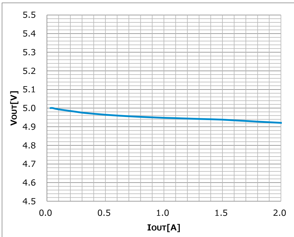
Figure 12. Load Regulation
