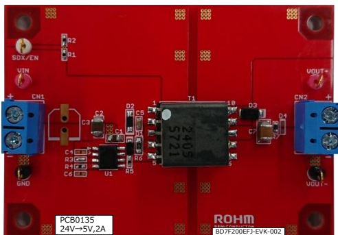
Figure 1. BD7F200EFJ-EVK-002 Evaluation Board
