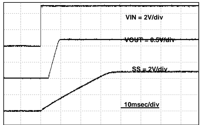
Fig.10 Soft start
