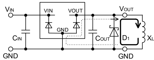
Figure 61. Current Path in Inductive Load (Output: Off)
