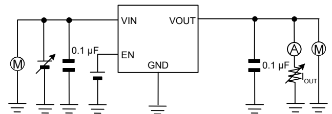
Measurement Setup for Figure 19 to 26, 41 to 48
