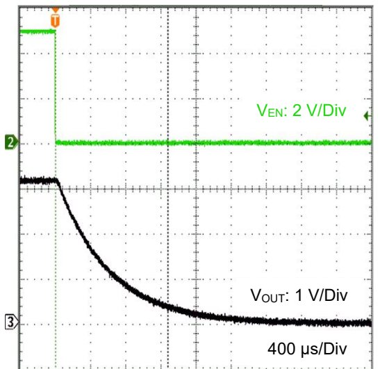
Figure 50. V_{EN} Shutdown Waveform (3.3 V output, I_{OUT} = 1\text{ mA} )
