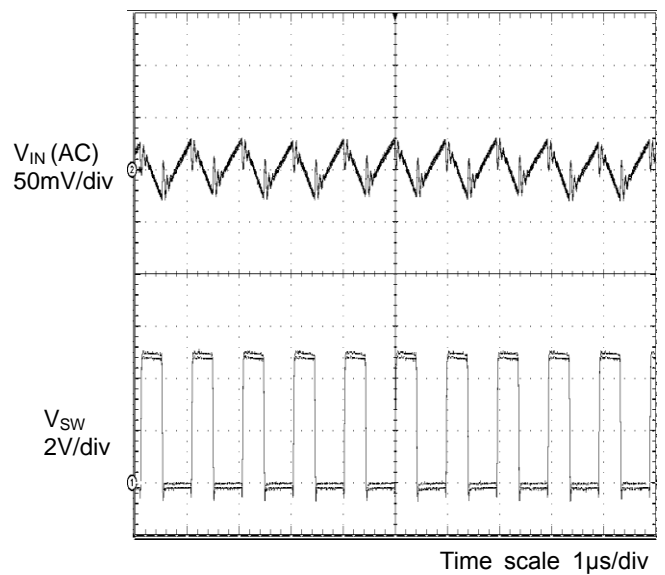
Figure 16. Input Voltage Ripple Wave V_{IN} = 5.0V , V_O = 1.8V , I_O = 1A
