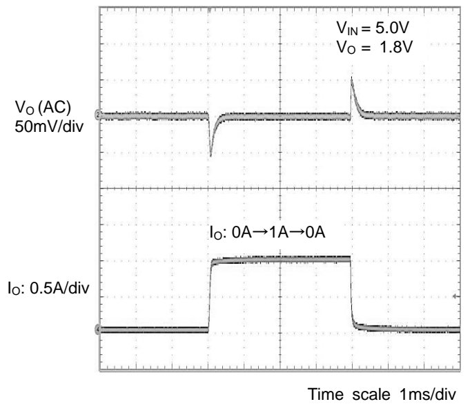
Figure 13. Load Transient Characteristics
