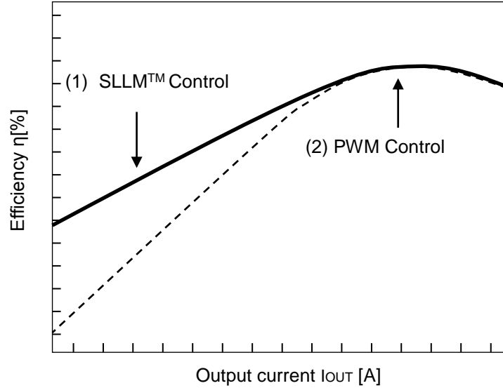
Figure 41. Efficiency (SLLM TM Control and PWM Control)
