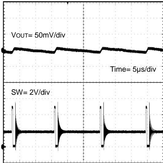
Figure 42. SW Waveform(SLLM TM Control) ( V_{in} = 5.0V, V_{out} = 1.8V, I_{out} = 50mA)
