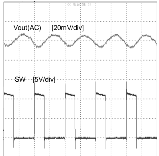
Figure 7. Vout Ripple (VIN=12V, Vout=3.3V, L=4.7μH, Cout=44μF, Iout=4A)
