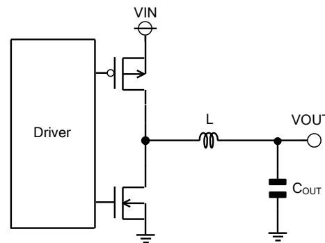
Figure 24. Output LC filter circuit
