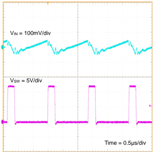
Figure 28. V_{IN} Ripple ( V_{IN} = 12V , V_{OUT} = 1.8V , I_{OUT} = 3A , L = 2.2\mu H , C_{OUT} = 22\mu F \times 2 )
