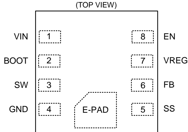
Figure 2. Pin Configuration
