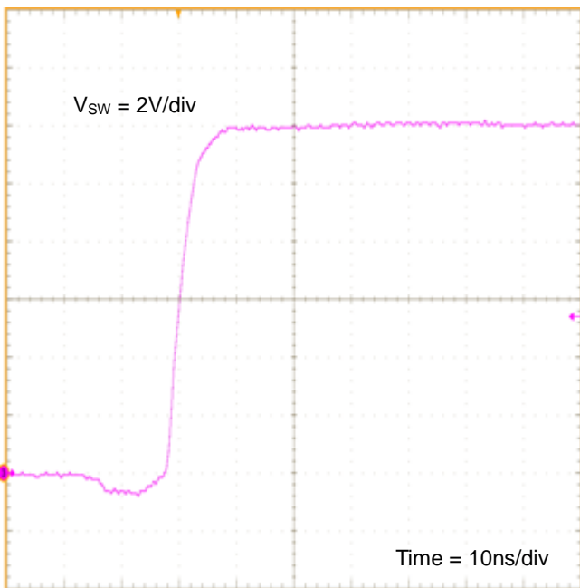
Figure 29. SW Turn ON ( V_{IN} = 12V , V_{OUT} = 1.8V , I_{OUT} = 3A , L = 2.2\mu H , C_{OUT} = 22\mu F \times 2 )
