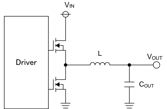
Figure 63. Output LC Filter Circuit
