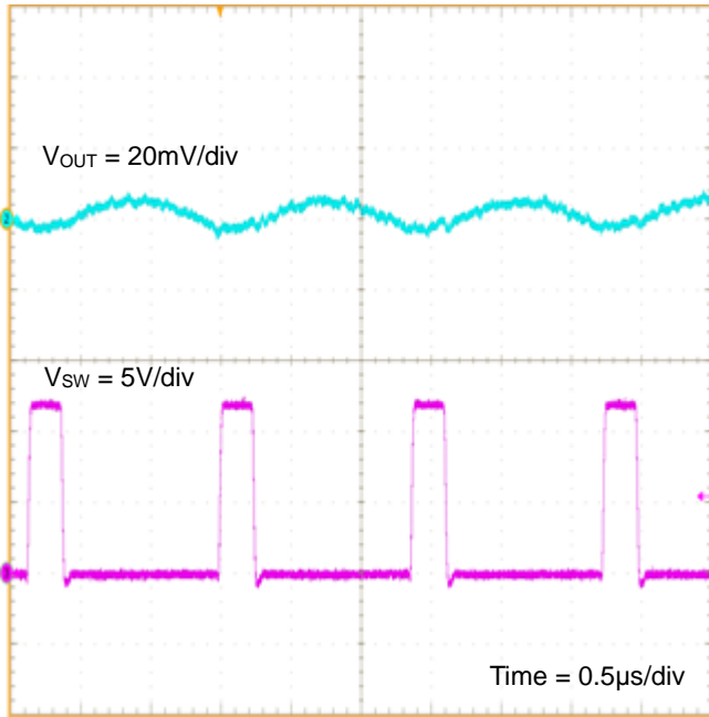
Figure 27. V_{OUT} Ripple ( V_{IN} = 12V , V_{OUT} = 1.8V , I_{OUT} = 3A , L = 2.2\mu H , C_{OUT} = 22\mu F \times 2 )
