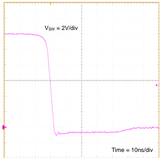
Figure 30. SW Turn OFF ( V_{IN} = 12V , V_{OUT} = 1.8V , I_{OUT} = 3A , L = 2.2\mu H , C_{OUT} = 22\mu F \times 2 )
