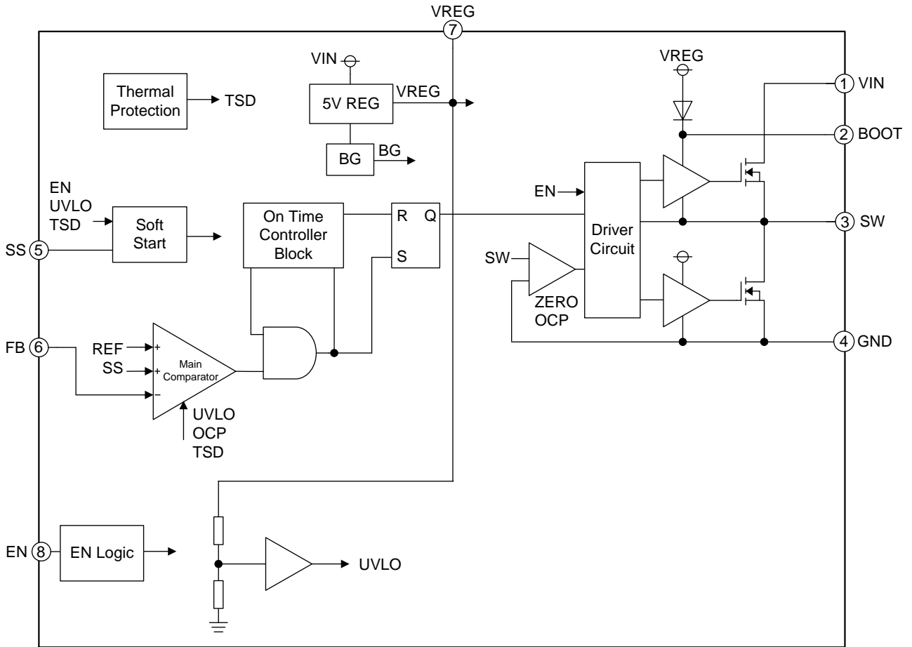
Figure 3. Block Diagram
