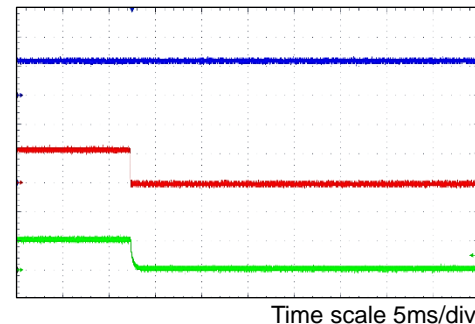
Figure 24. Power-down by EN V_{IN} = 12V, V_O = 5.0V, I_O = 0A
