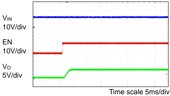
Figure 23. Start-up by EN V_{IN} = 12V, V_O = 5.0V, I_O = 0A
