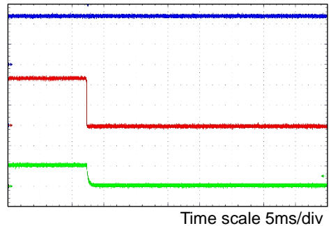
Figure 26. Power-down by EN V_{IN} = 24V, V_O = 5.0V, I_O = 0A
