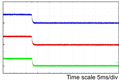
Figure 20. Power-down EN = V_{IN} V_{IN} = 12V, V_O = 5.0V, I_O = 0A
