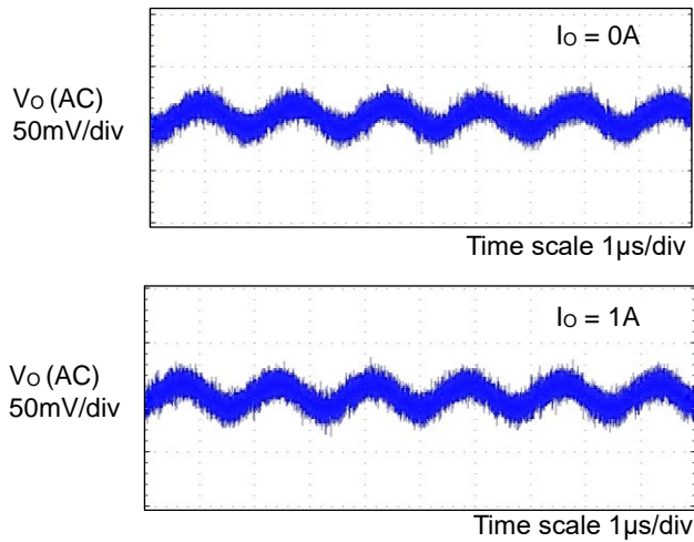
Figure 17. Output Voltage Ripple Wave V_{IN} = 12V, V_O = 5.0V
