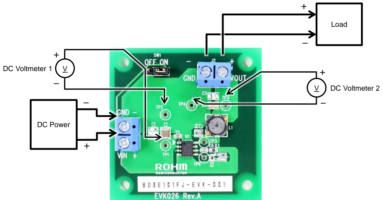
Figure 1. Connection Diagram
