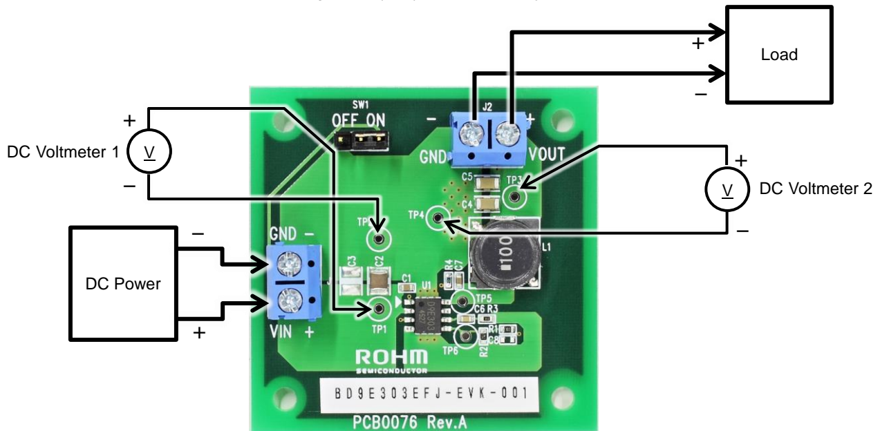
Figure 1. Connection Diagram
