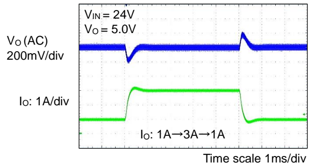
Figure 12. Load Transient Characteristics
