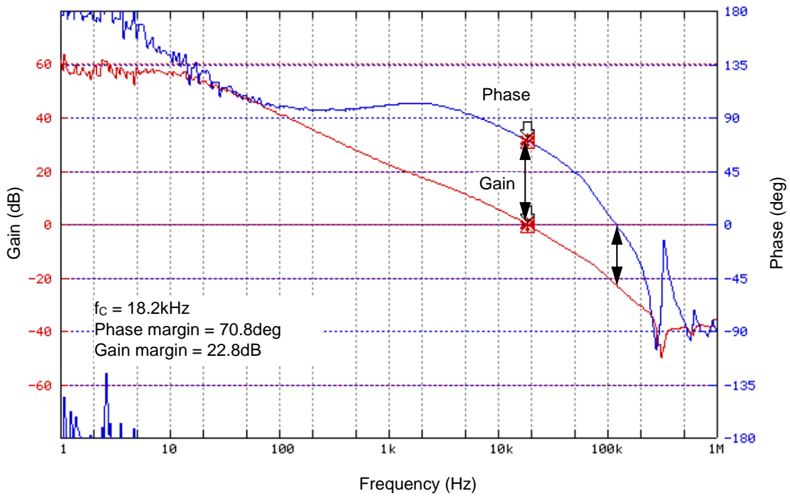
Figure 14. Loop Response V_{IN} = 24\text{V} , V_O = 5.0\text{V} , I_O = 3\text{A}
