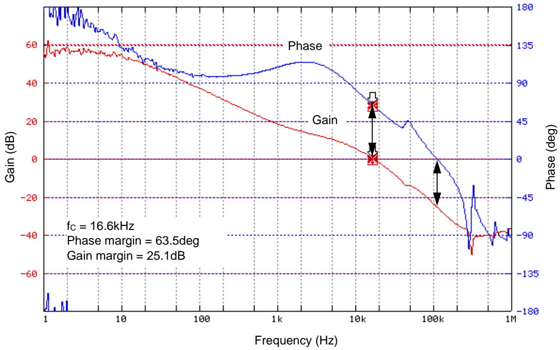
Figure 13. Loop Response V_{IN} = 12\text{V} , V_O = 5.0\text{V} , I_O = 3\text{A}
