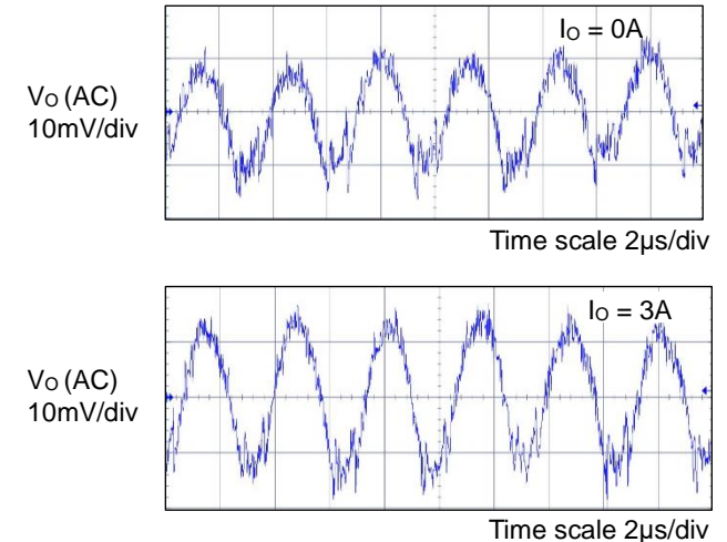
Figure 18. Output Voltage Ripple Wave V_{IN} = 24V, V_O = 5.0V
