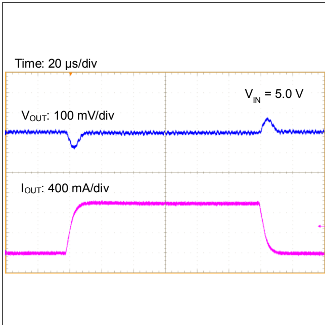
Figure 36. Load Transient Response ( I_{OUT}=0\text{ A}\leftrightarrow 1\text{ A} )
