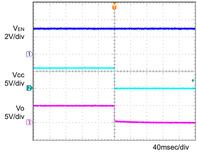
Figure 12. OFF sequence 1 C_o = 1\mu\text{F} , T_a = -40^\circ\text{C}
