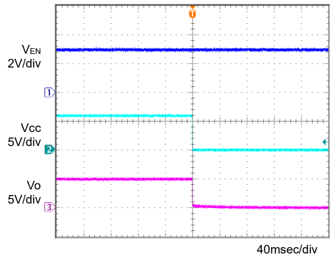
Figure 14. OFF sequence 1 C_o = 1\mu\text{F} , T_a = 105^\circ\text{C}
