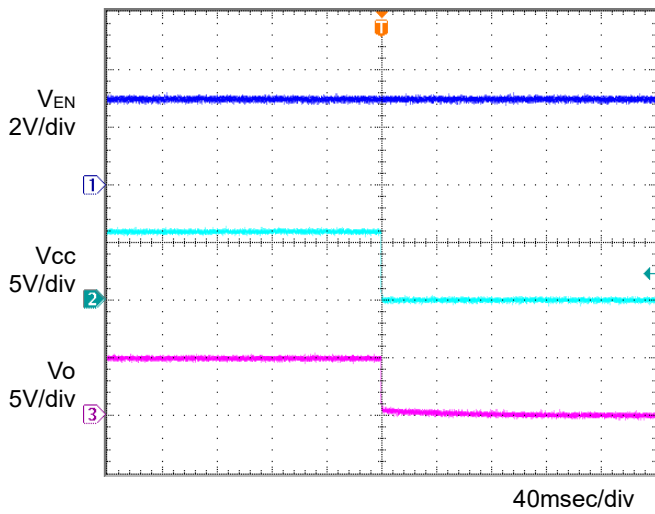
Figure 13. OFF sequence 1 C_o = 1\mu\text{F} , T_a = 25^\circ\text{C}
