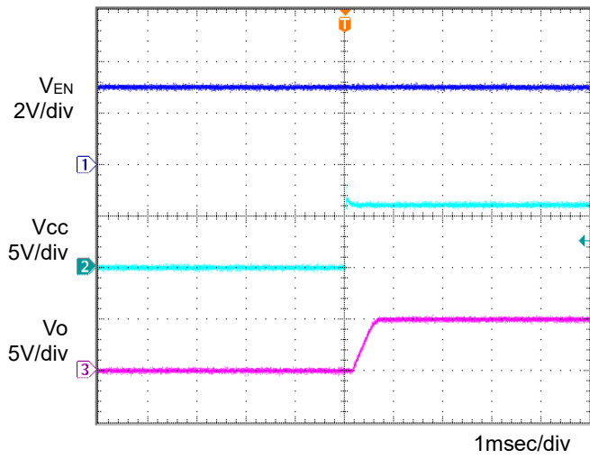
Figure 11. Input sequence 1 C_o = 1\mu\text{F} , T_a = 105^\circ\text{C}
