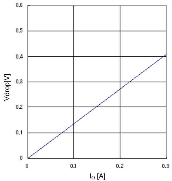
Figure 22. Minimum dropout Voltage 2 ( V_{CC}=4.5 V, T_a=25^\circ C )
