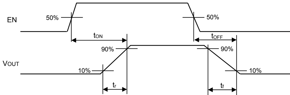
Figure.6 Timing diagram
