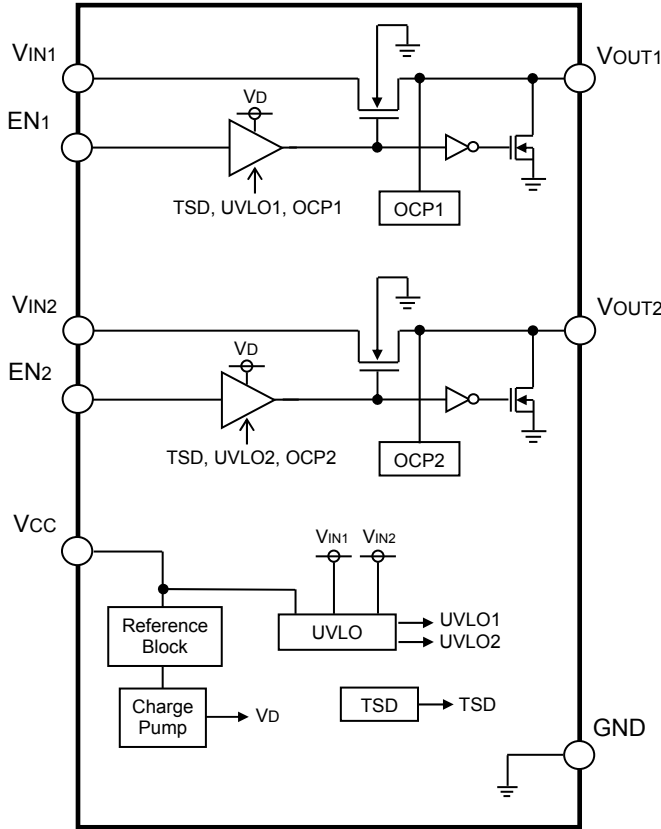
Figure.3 Block diagram
