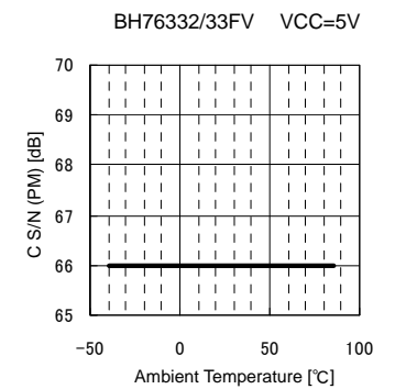
Fig.100 SN_{CP} vs. Ambient Temperature
