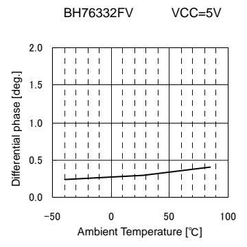
Fig.92 DP vs. Ambient Temperature
