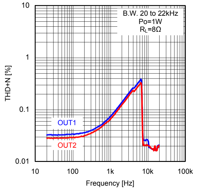
Figure 19. THD+N - Frequency
