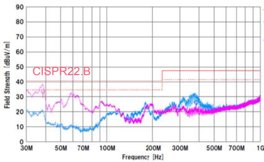
Figure 23. Radiated Emission.1
