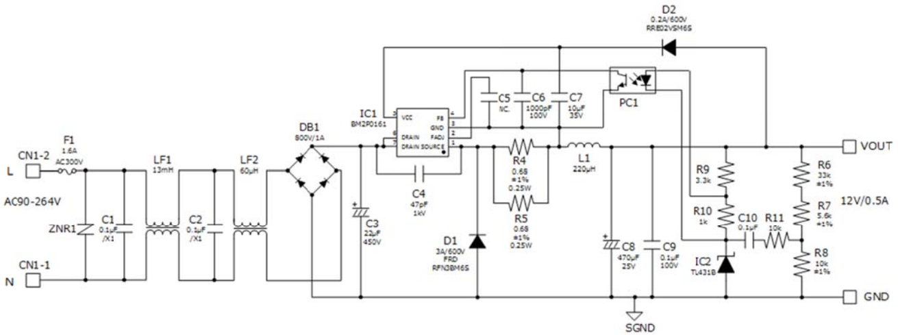
Figure 3. BM2P0161-EVK-002 Schematics
