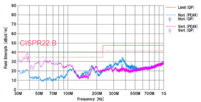
Figure 24. Radiated Emission.2
