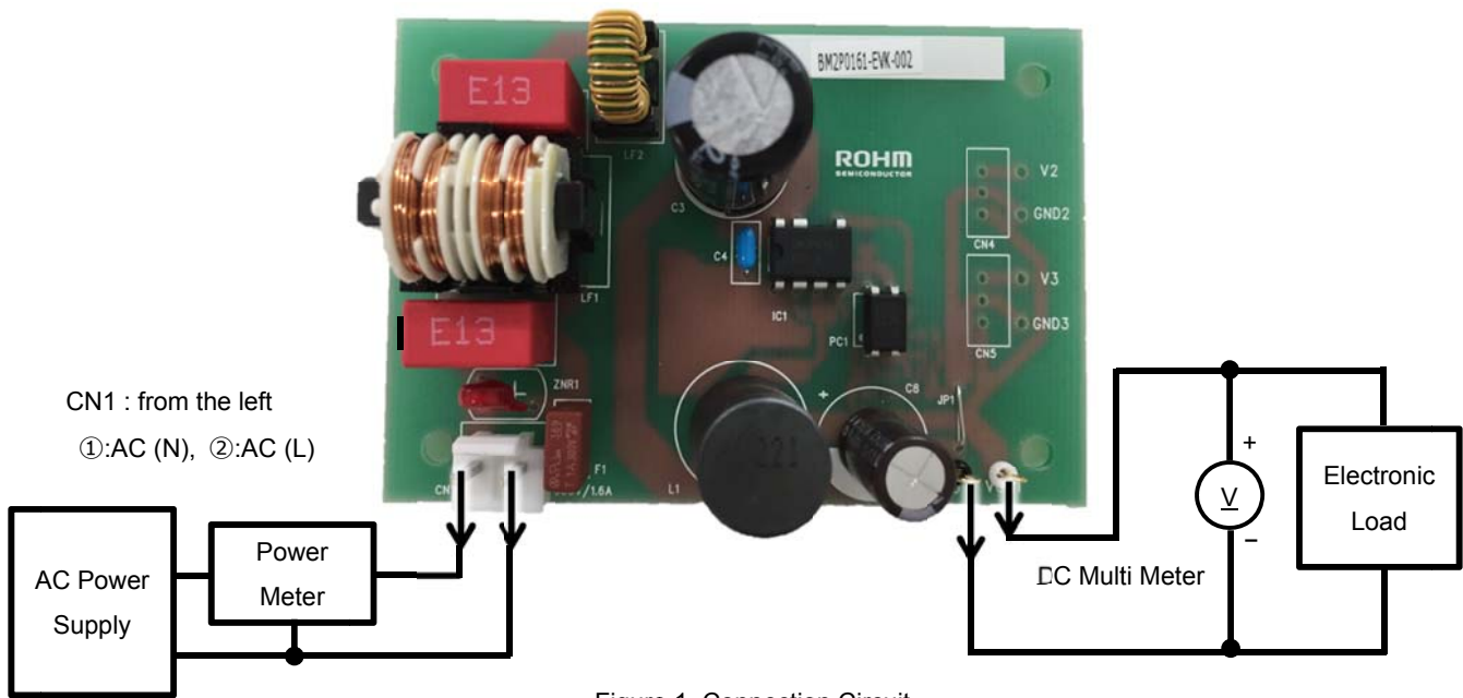
Figure 1. Connection Circuit
