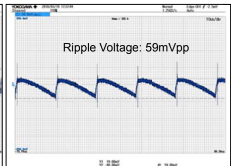
Figure 20. VOUT Ripple Voltage.6 V_{IN}=230Vac , I_{OUT}=500mA CH1: VOUT 50mV/div, 10μs/div
