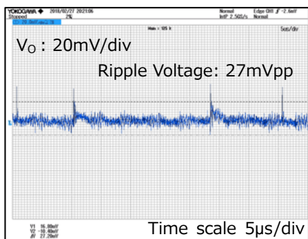
V_{IN}=100Vac , I_{OUT}=10mA
