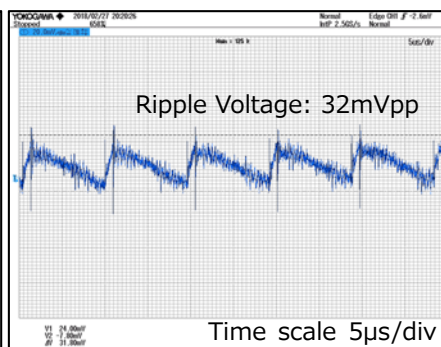
V_{IN}=100Vac , I_{OUT}=167mA
