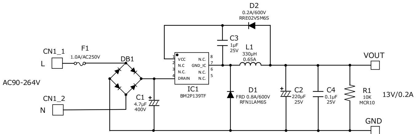
Figure 3. BM2P139TF-EVK-001 Schematics
