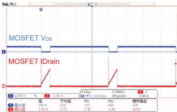
Figure 16. MOSFET V_{IN} = 90 \text{ Vac} , I_{OUT} = 0.8 \text{ A}
