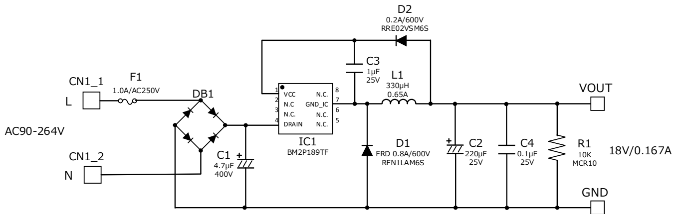
Figure 3. BM2P189TF-EVK-001 Schematics
