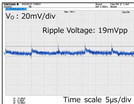
V_{IN}=100Vac , I_{OUT}=10mA
