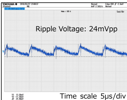
V_{IN}=100Vac , I_{OUT}=100mA
