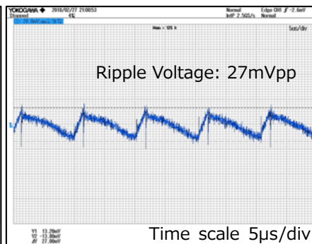
V_{IN}=100Vac , I_{OUT}=167mA
