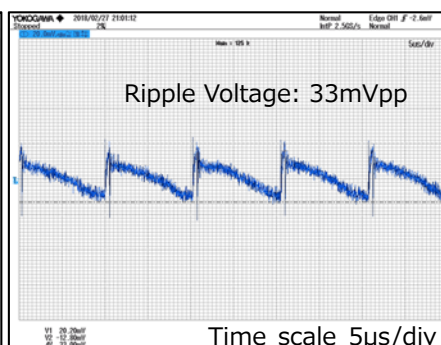
V_{IN}=230Vac , I_{OUT}=167mA
