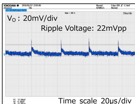
V_{IN}=230Vac , I_{OUT}=10mA
