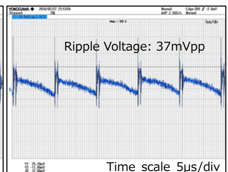
V_{IN}=230Vac , I_{OUT}=150mA
