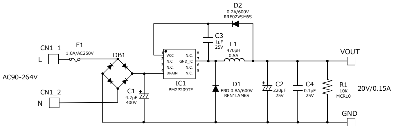
Figure 3. BM2P209TF-EVK-001 Schematics
