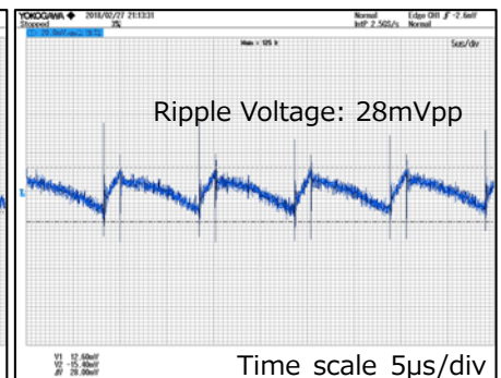
V_{IN}=100Vac , I_{OUT}=150mA
