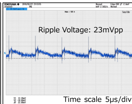
V_{IN}=100Vac , I_{OUT}=50mA
