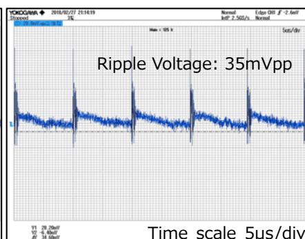
V_{IN}=230Vac , I_{OUT}=50mA
