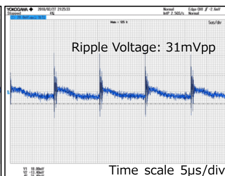
V_{IN}=230Vac , I_{OUT}=50mA
