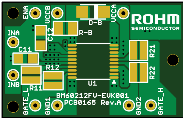
Silkscreen (Top)
