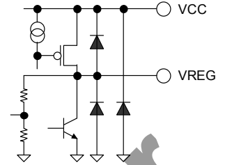
Figure 50. VREG, VCC
