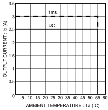
Fig.12 Derating curve
