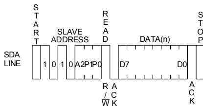
Figure 38. Current Read Cycle
