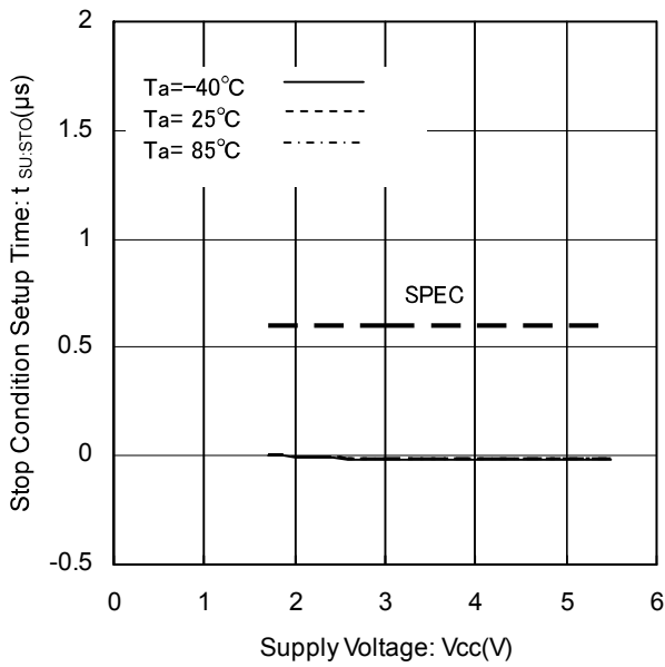
Figure 24. Stop Condition Setup Time vs Supply Voltage
