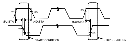
Figure 2-(b). Start-stop Bit Timing
