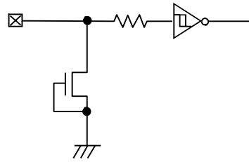
Figure 49. Input Pin Circuit Diagram
