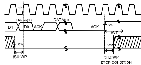
Figure 2-(d). WP Timing at Write Execution
