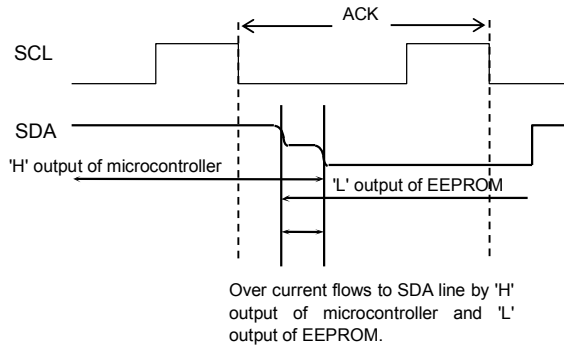
Figure 46. Input / Output Collision Timing
