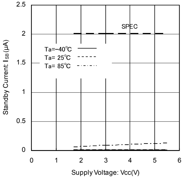
Figure 12. Standby Current vs Supply Voltage
