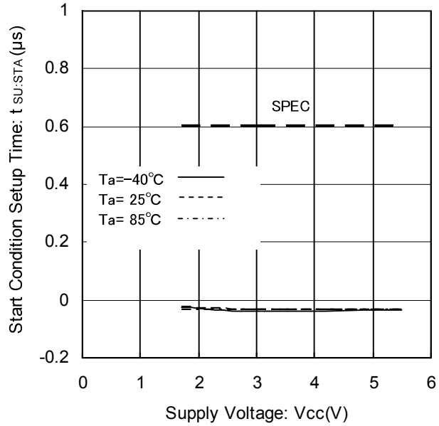
Figure 17. Start Condition Setup Time vs Supply Voltage
