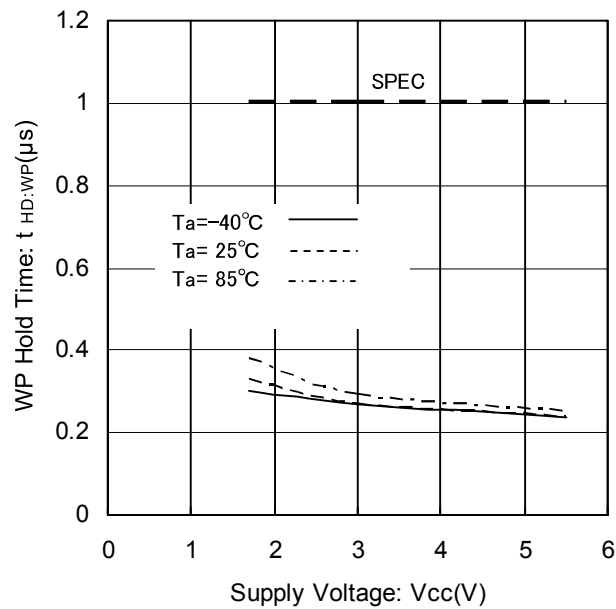
Figure 31. WP Hold Time vs Supply Voltage
