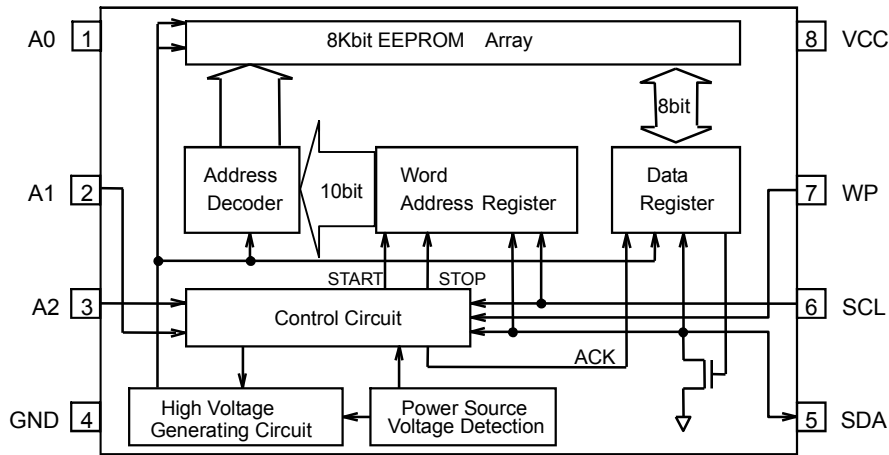
Figure 3. Block Diagram
