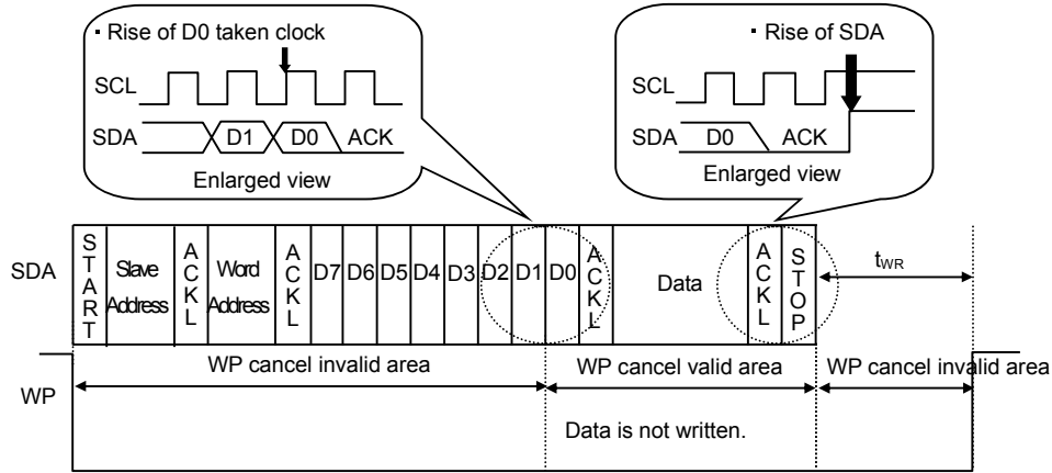
Figure 42. WP Valid Timing
