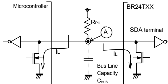
Figure 44. I/O Circuit Diagram
