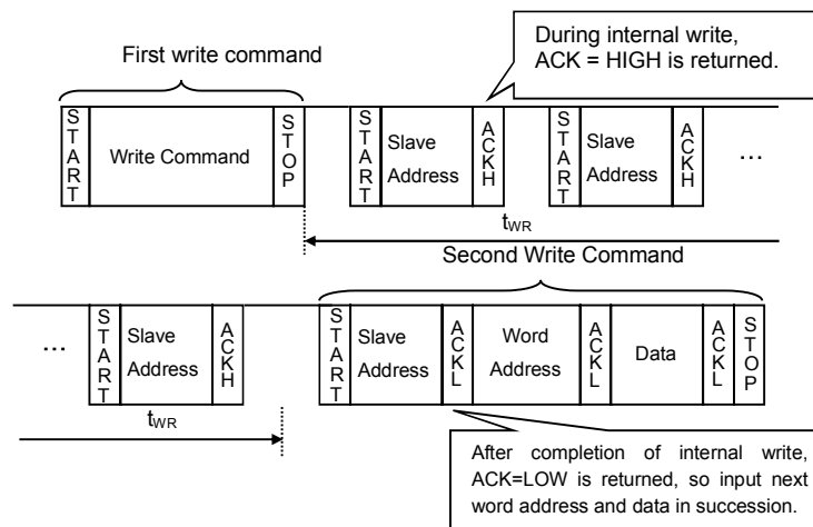
Figure 41. Case of Continuous Write by Acknowledge Polling
