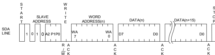
Figure 36. Page Write Cycle
