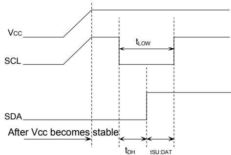
Figure 52. When SCL= 'H' and SDA= 'L'
