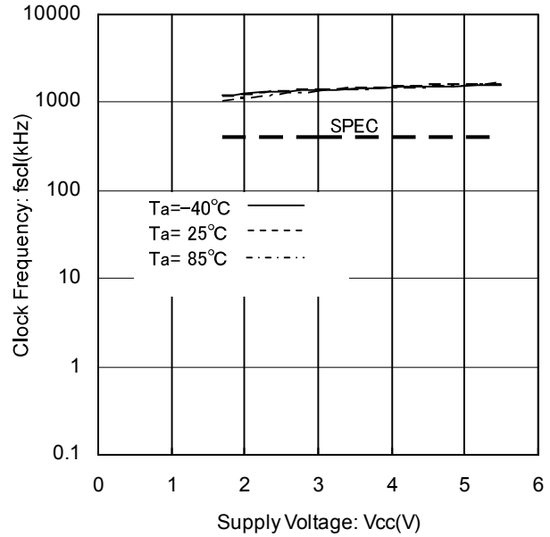
Figure 13. Clock Frequency vs Supply Voltage
