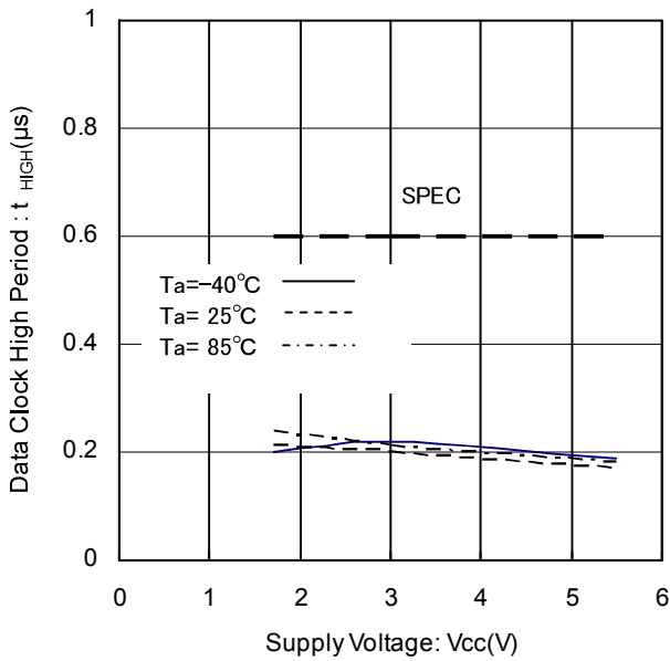
Figure 14. Data Clock High Period vs Supply Voltage
