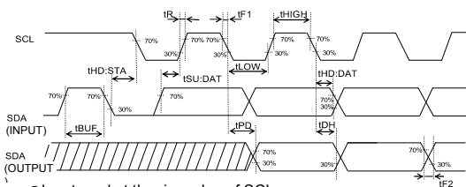
Figure 2-(a). Serial Input / Output Timing
