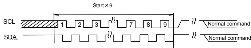
Figure 40-(c). START×9 + Command Input
