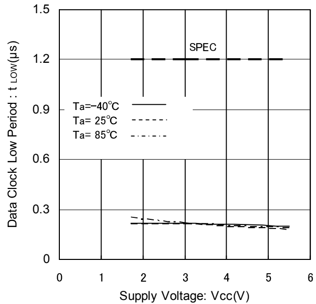
Figure 15. Data Clock Low Period vs Supply Voltage
