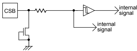
Figure 48. CSB input equivalent circuit
