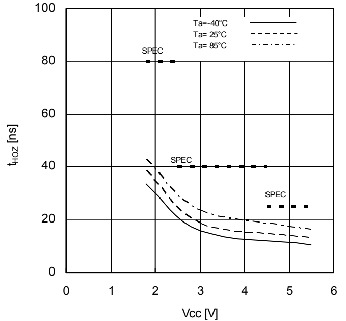
Figure 31. Time from HOLDB to Output High-Z vs Supply Voltage
