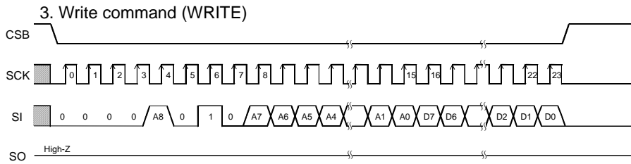
Figure 38. Write command
