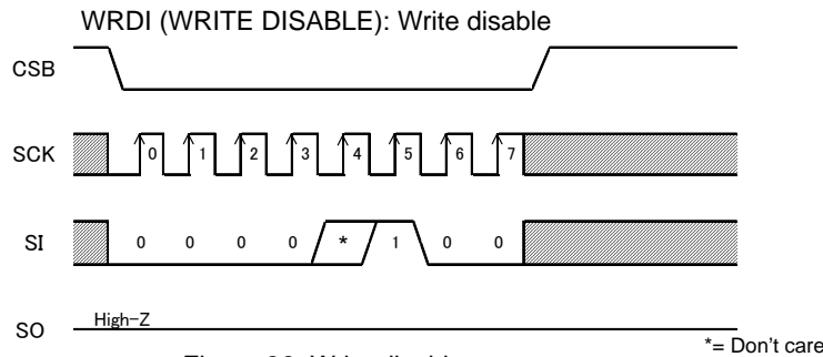
Figure 36. Write disable
