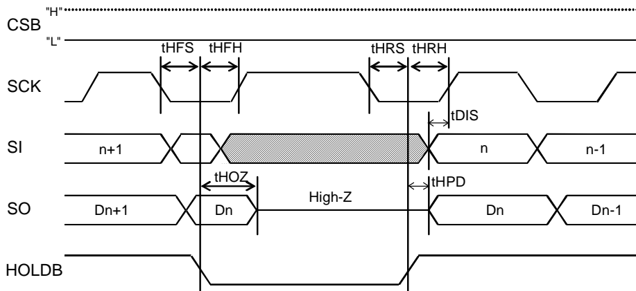
Figure 4. HOLD timing
