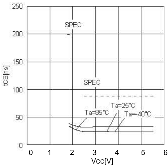
Figure 18. \overline{CS} high time tCS
