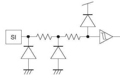
Figure 58. SI input equivalent circuit
